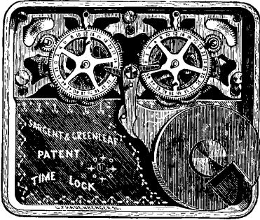
CUT OF BANK LOCK.
