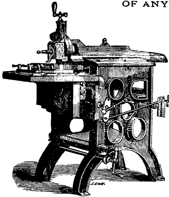
SHAPING PLANER. Planes 12 x 18 inches; has quick return motion.
