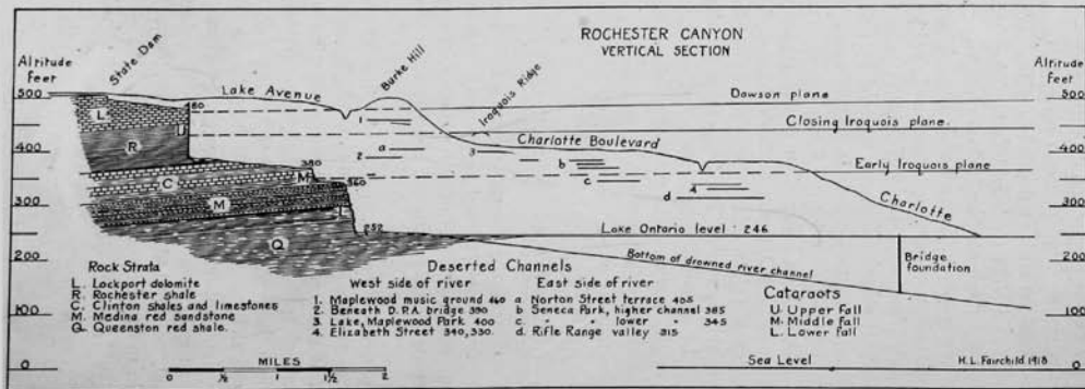
FIGURE 11. Vertical Section of the Rochester Canyon.
