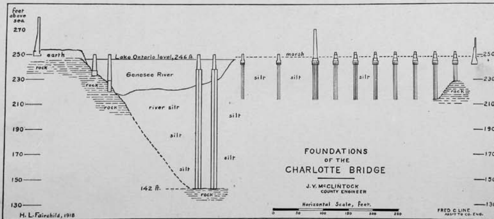
FIGURE 10. Drowned Channel of the Genesee River
