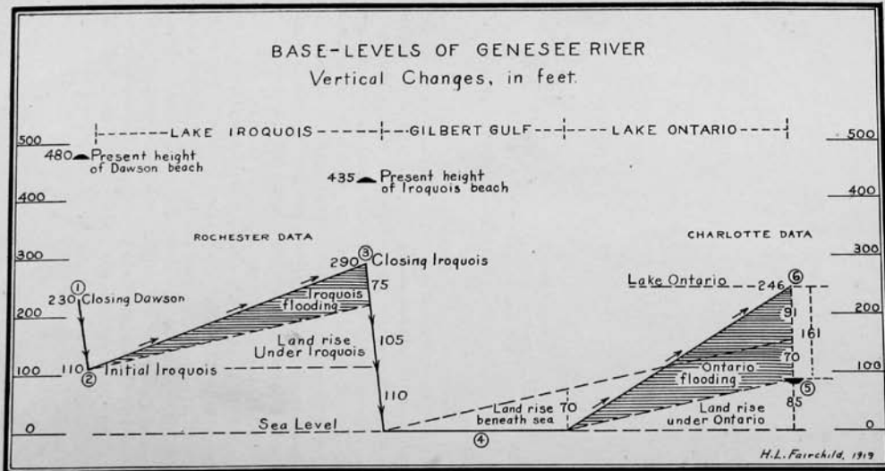
FIGURE 8. Vertical Changes in the Genesee River Base-Levels
