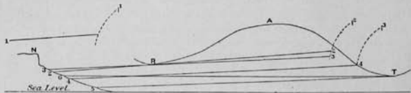
PLATE III.—Diagram to illustrate the relations of Water Levels in the Ontario Basin to attitudes of the land and to outlets.
