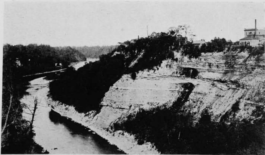
ROCK STRATA, ROCHESTER CANYON
